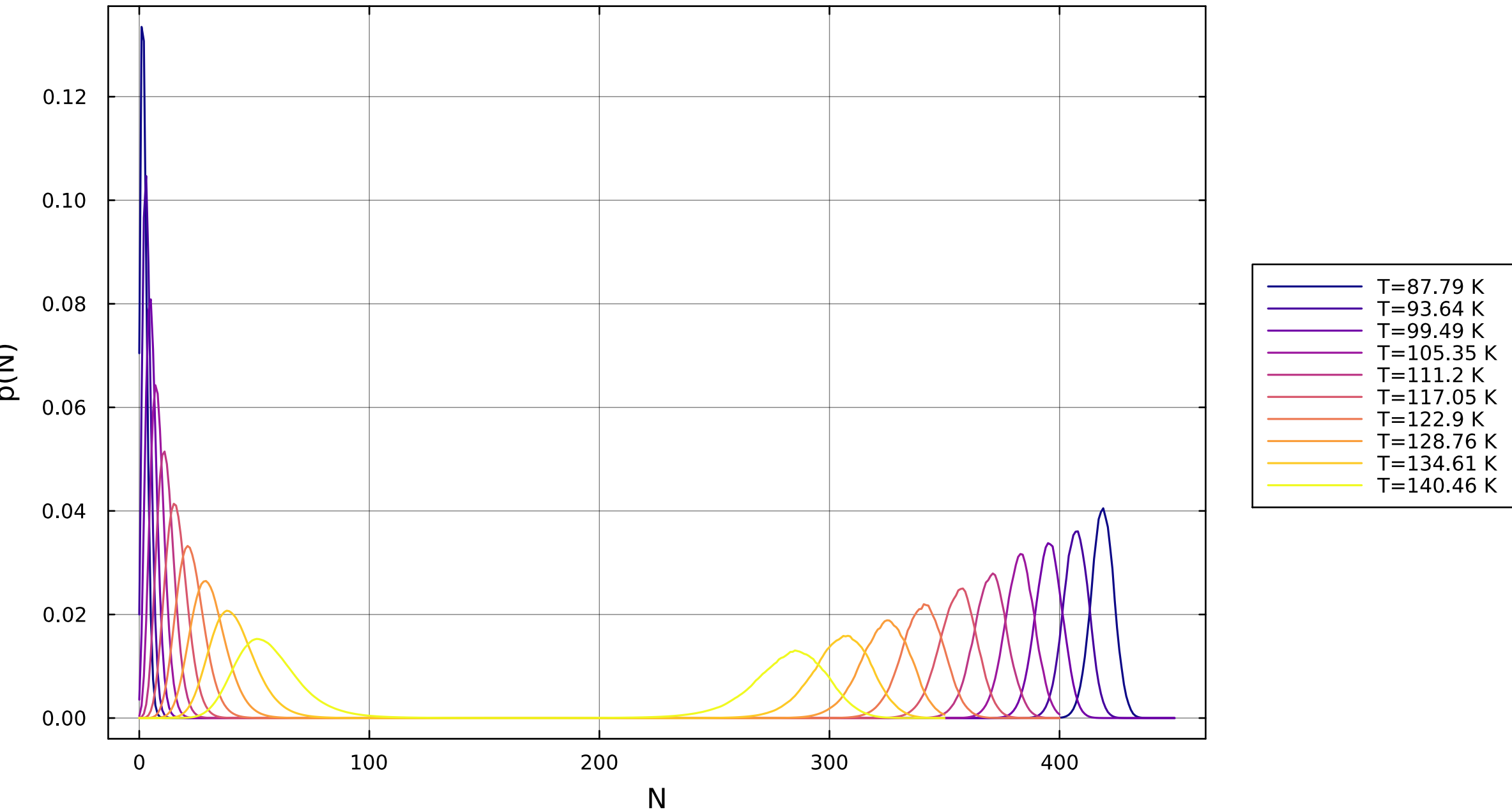
p(N) at coexistence — all temperatures
