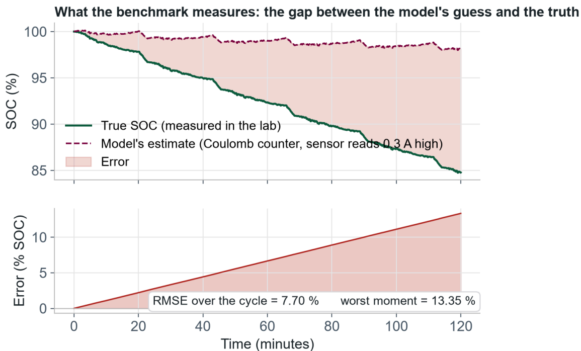
Figure 1.7 Estimation error is the difference between the model's estimate and the reference state of charge. Here a Coulomb-counting model fed a biased current measurement drifts steadily from the reference; the shaded band is what the benchmark quantifies.
