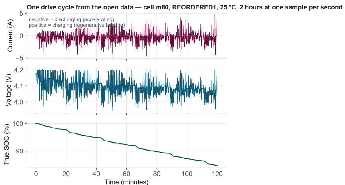
Figure 1.3 Two hours of one drive cycle from the open dataset. Current alternates between discharge and regenerative charge with every acceleration and braking event; voltage responds to it; the reference state of charge declines from full. A model receives the current, voltage and temperature and must reproduce the state-of-charge trace.
