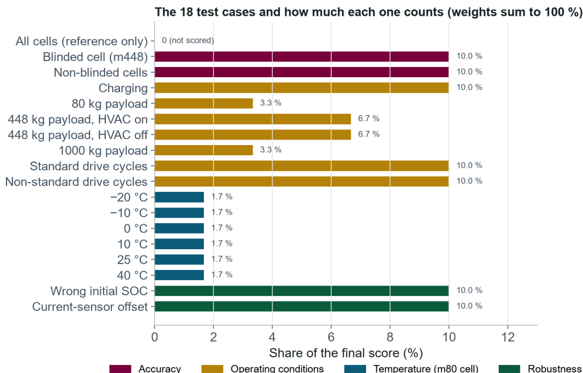
Figure 5.3 The eighteen test cases and their weights. Robustness and generalisation are weighted as heavily as raw accuracy.
