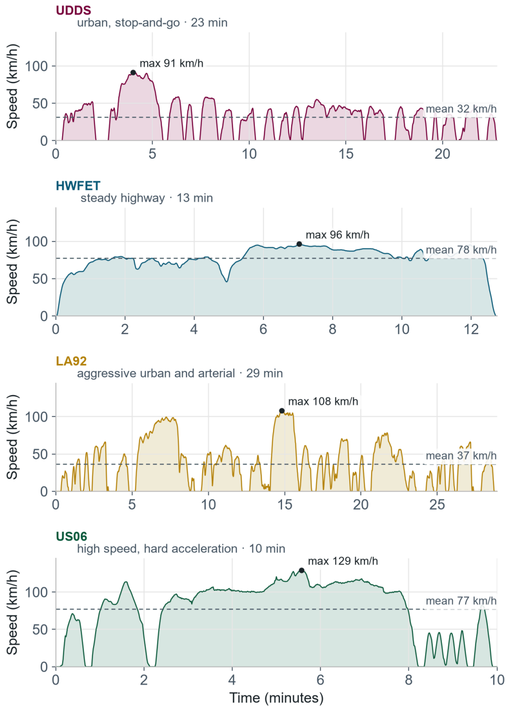
Figure 1.2 The four standard drive cycles as speed profiles. UDDS and LA92 are urban, with frequent stops; HWFET and US06 are sustained high-speed driving. Each profile was converted to the current a Model 3 cell would deliver while following it.
