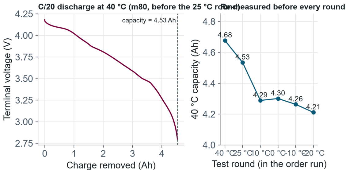
Figure 1.5 The capacity reference. Left: the C/20 discharge at 40 °C recorded before the 25 °C round, which defines 4.53 Ah as that round's capacity. Right: the same measurement repeated before every round, showing the cell losing about 10 % of its capacity over the eight-month campaign.
