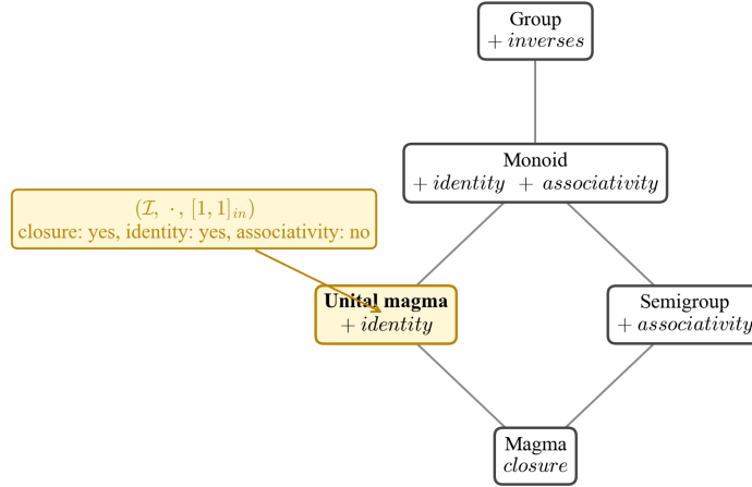
Algebraic structures with one binary operation (arrows denote “adds an axiom” — strictly stronger structure)
