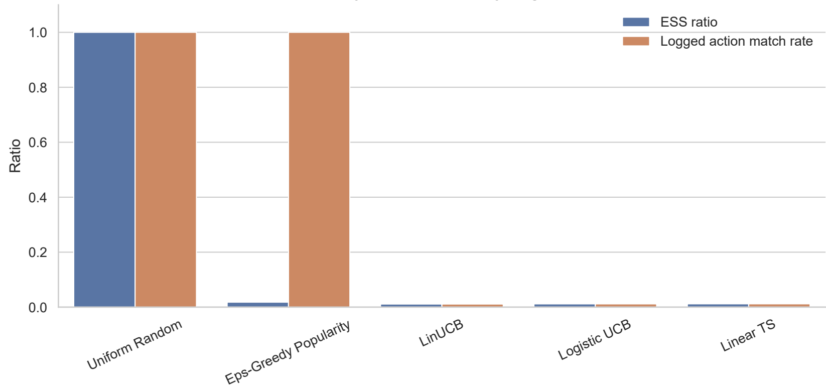
Off-Policy Evaluation Stability Diagnostics
