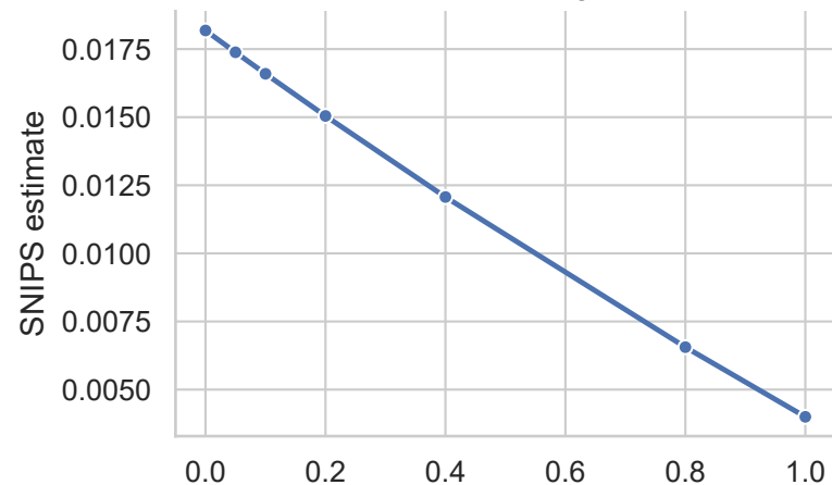
Eps-Greedy
