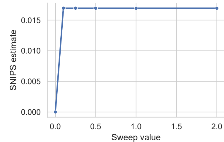
Logistic UCB
