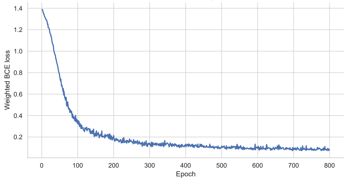
Reward Model Training Loss
