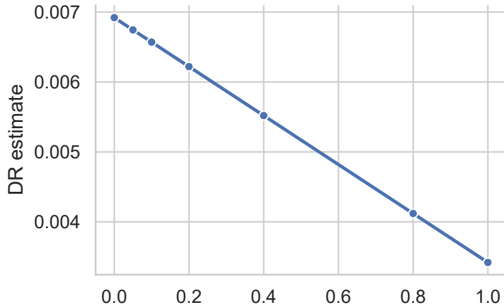
Logistic UCB
