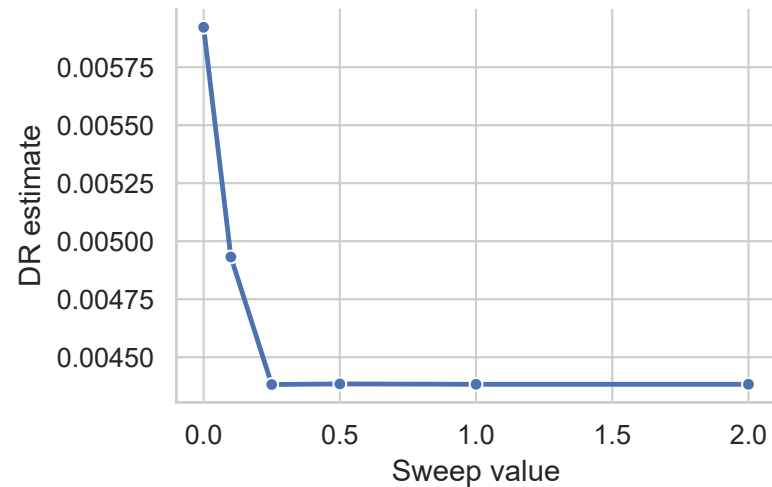
Logistic UCB
