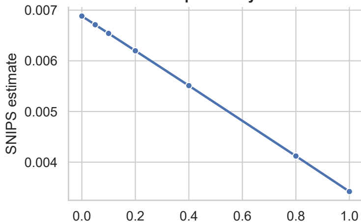
Logistic UCB
