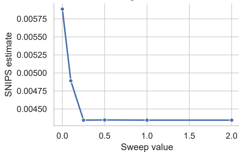
Logistic UCB
