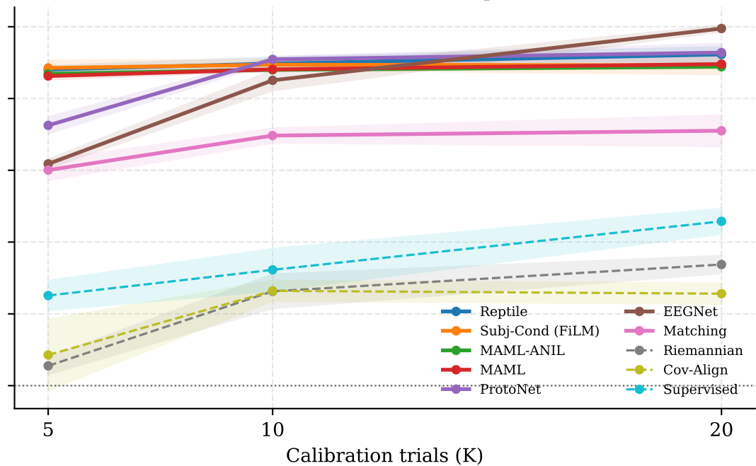
Cross-dataset (ErrP-Coadaptation)
