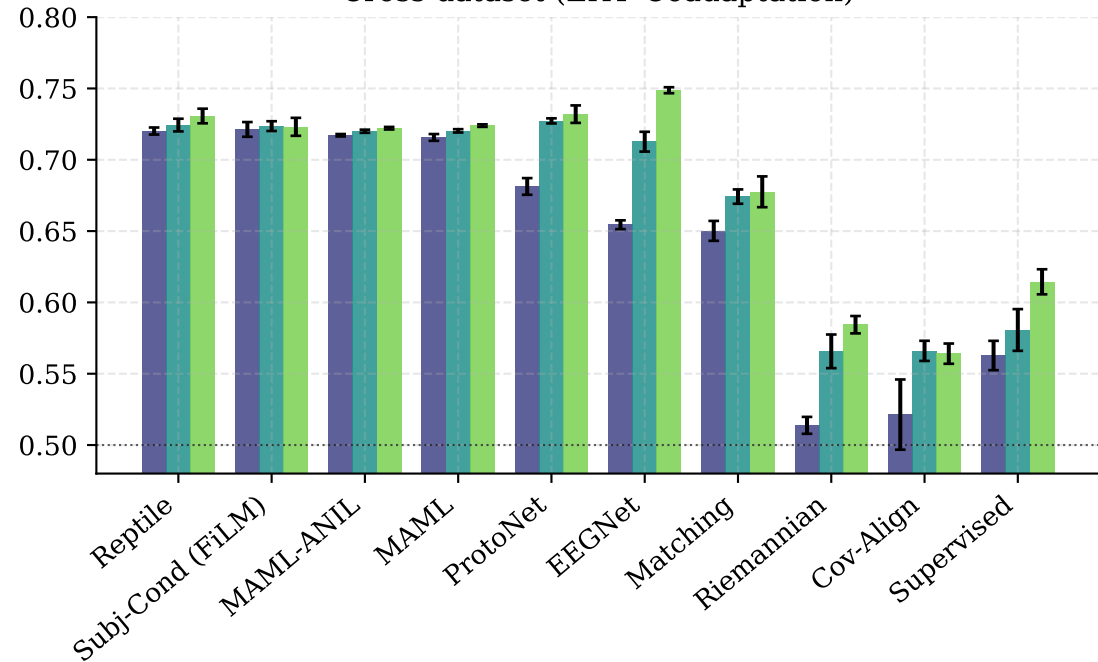
Cross-dataset (ErrP-Coadaptation)
