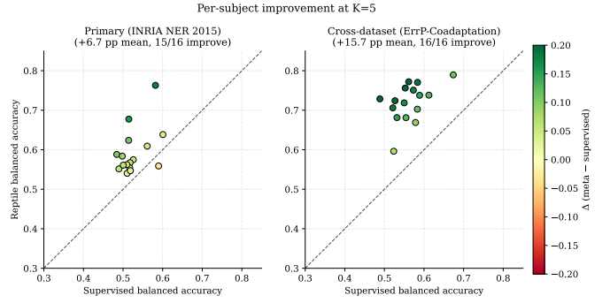
Fig. 1. Per-subject balanced accuracy at K=5 : Reptile vs. supervised. Points above the diagonal are subjects where meta-learning helps; color encodes the gain.
