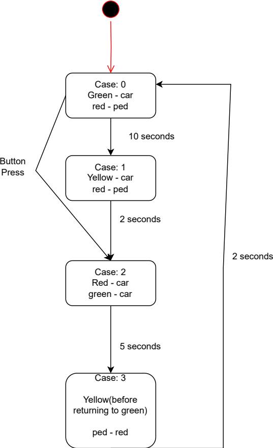
State Machine Diagram
