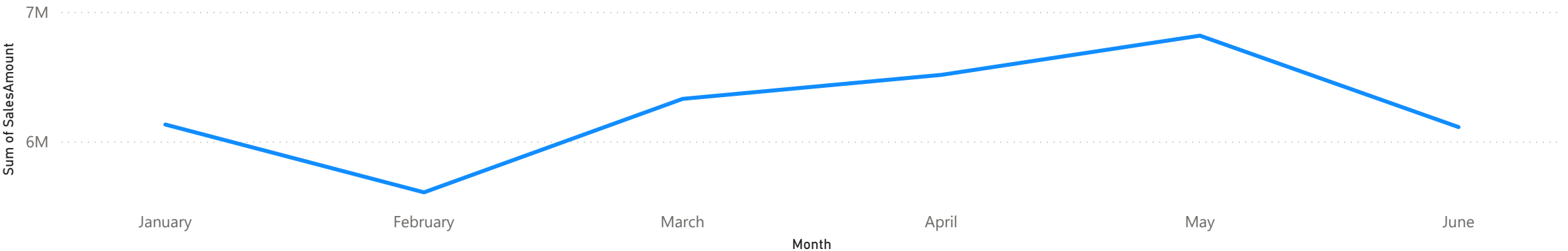
Sales Trend Over Time
