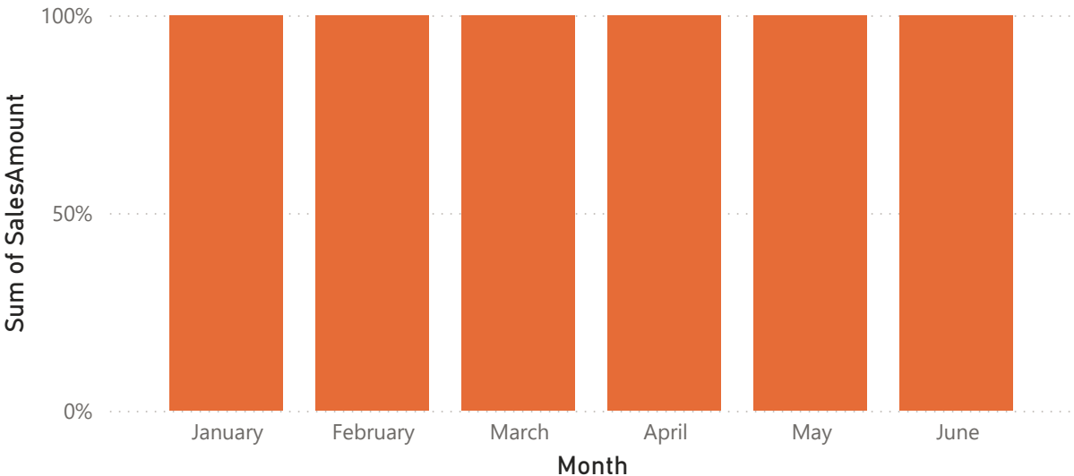
Sum of SalesAmount by Month
