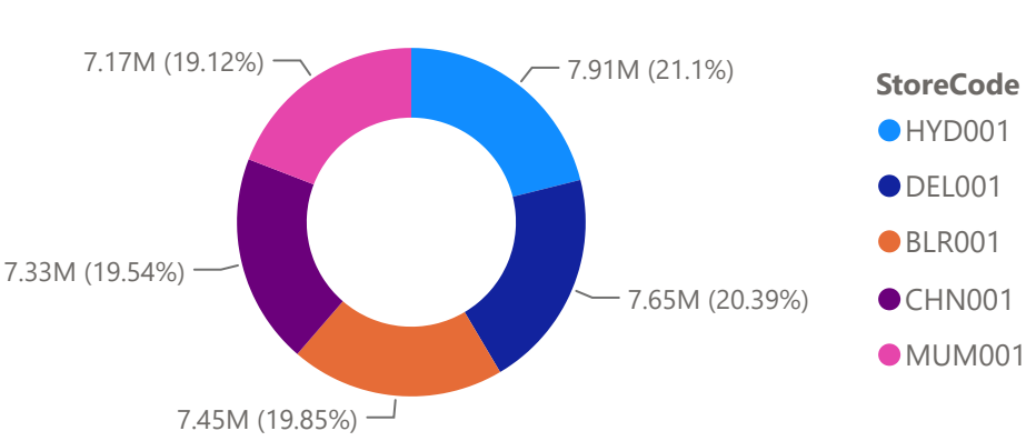
Sales by Store
