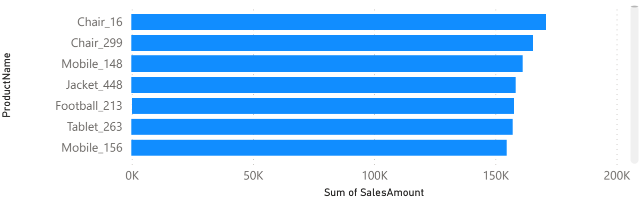
Top Products by Sales
