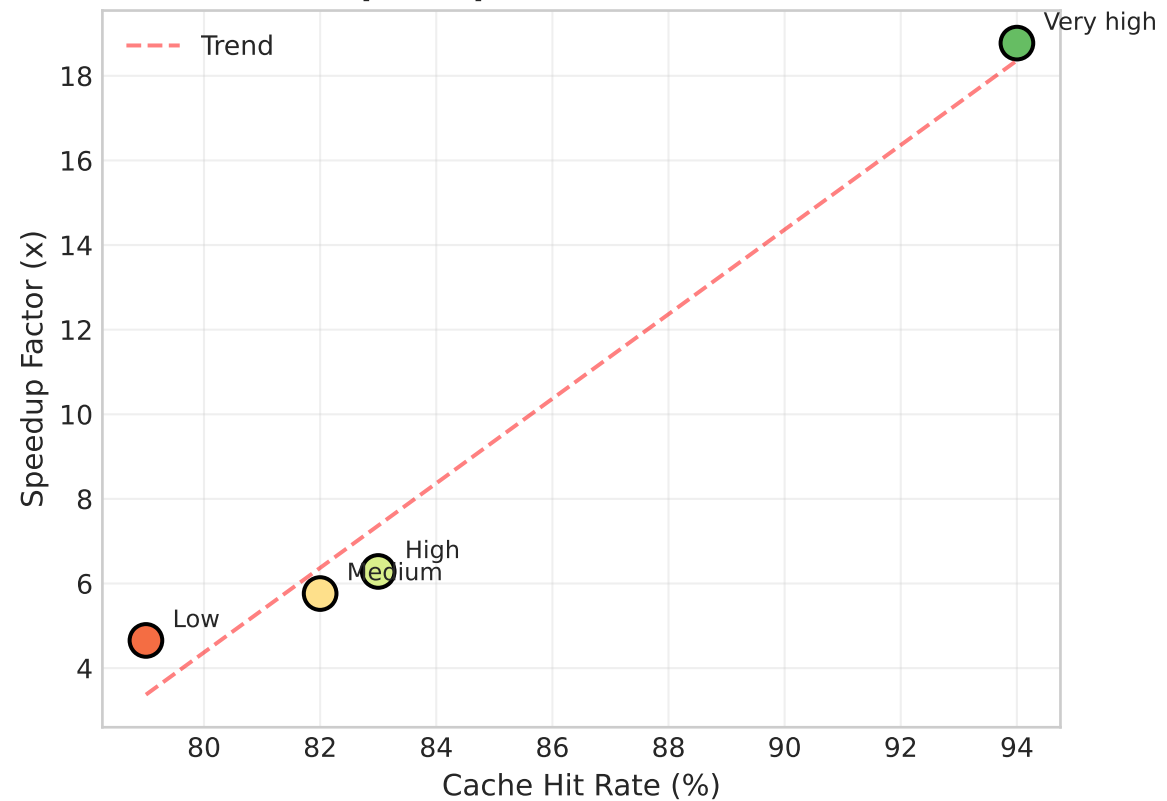
Speedup vs Cache Hit Rate
