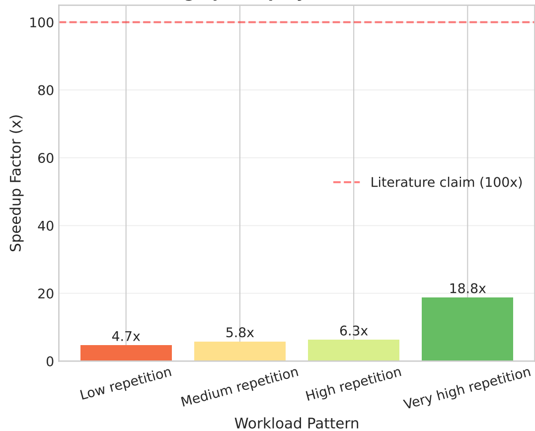
Caching Speedup by Workload Pattern
