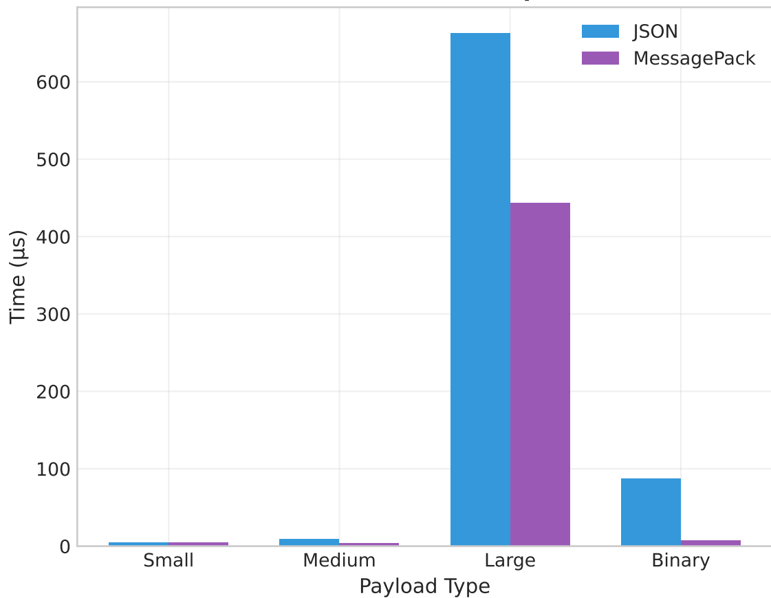
Serialization Round-trip Time
