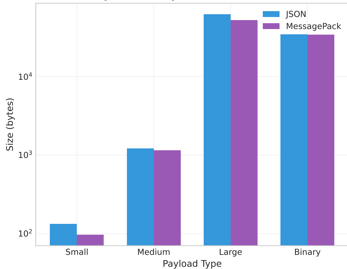
Payload Size by Serialization Format
