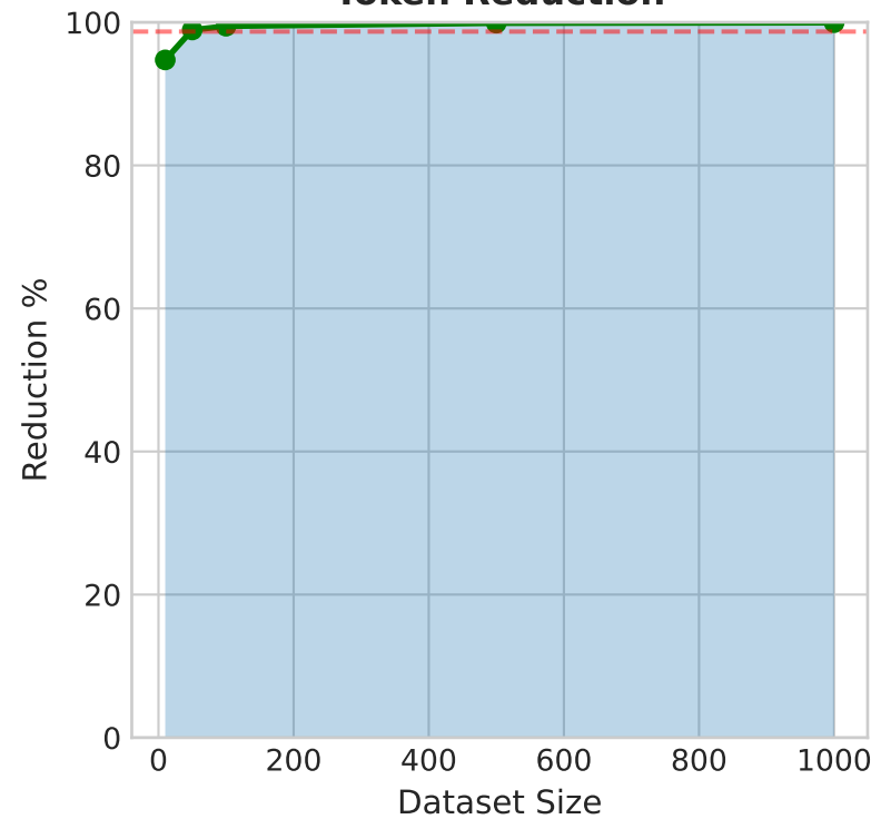
Token Reduction
