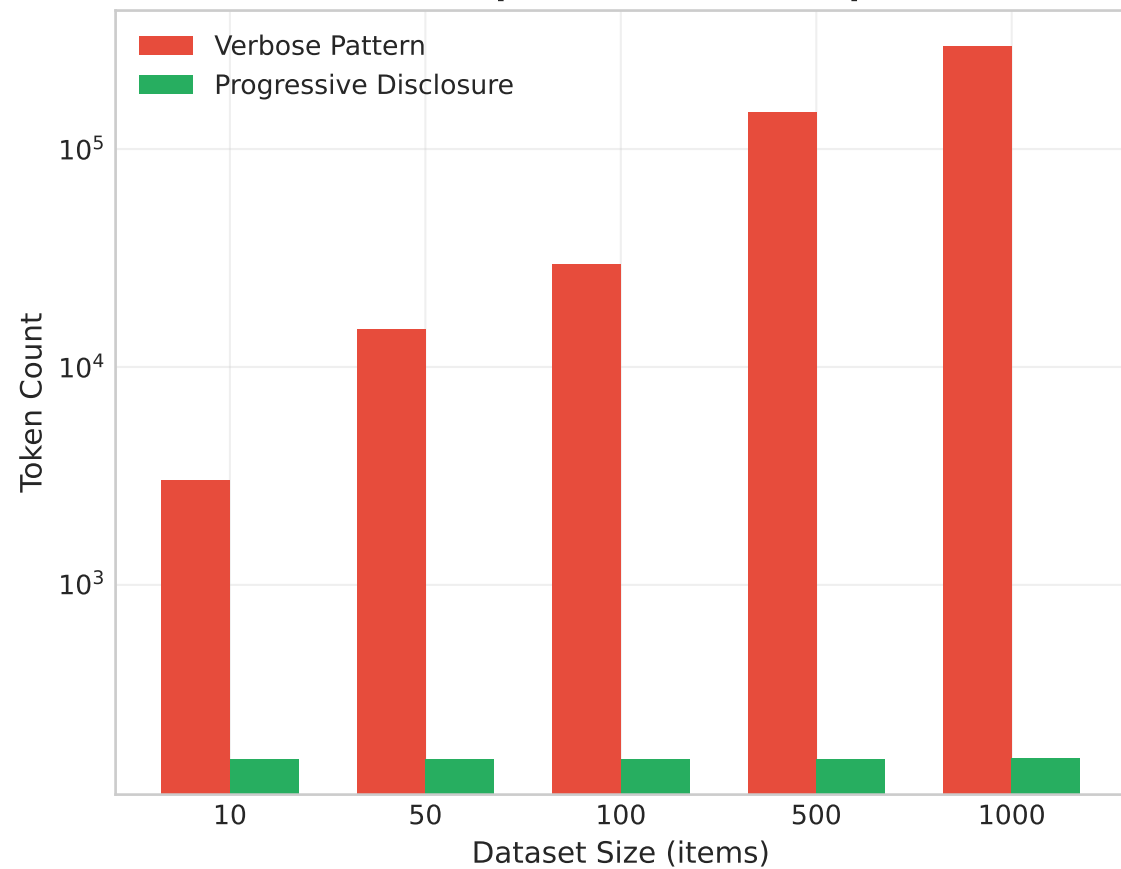
Token Consumption: Verbose vs Optimized
