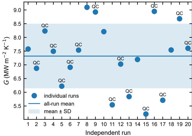
(a) Interfacial thermal conductance
