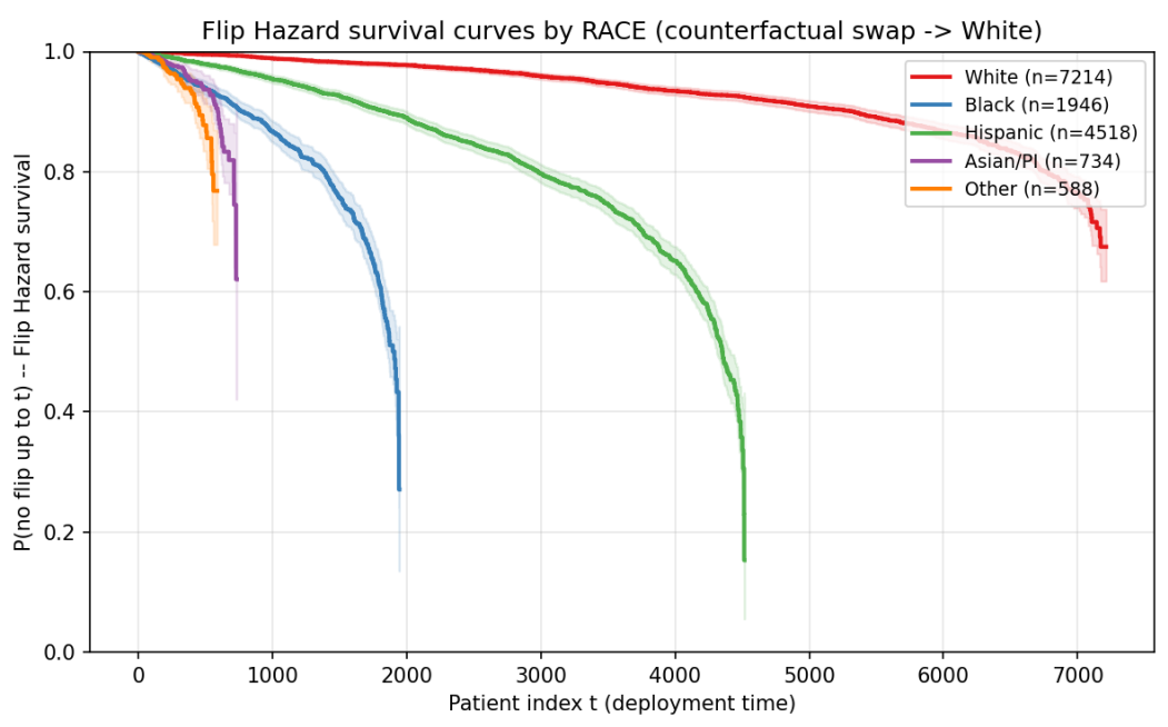
Fig. 6. Section 6.4. Group-stratified Flip Hazard no-flip survival at n = 15\,000 . Greenwood 95% bands shown.
