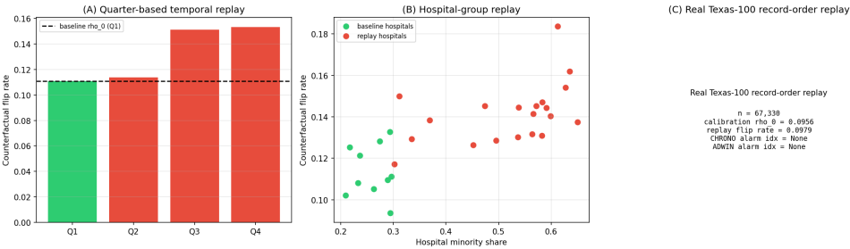
Fig. 21. Section 6.14. Replay streams. (A) Per-quarter flip rate, with the Q3 drift onset. (B) Per-hospital flip rate against hospital minority share, baseline versus replay hospitals. (C) Real Texas-100 record-order replay summary.
