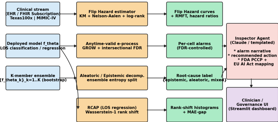
CHRONO-Fair: Counterfactual Hazard-Rate ONLINE Surveillance of Fairness
