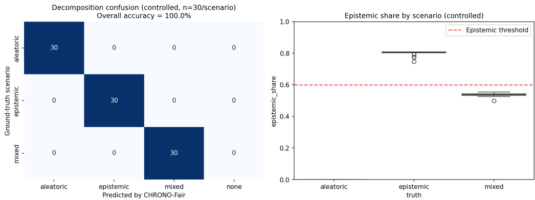
Fig. 3. Section 6.3 Track 1. Controlled decomposition validation, 30 trials per scenario at n = 1000 . Confusion matrix on the left; per-scenario epistemic share on the right. The 0.6 threshold is the Inspector Agent decision boundary.
