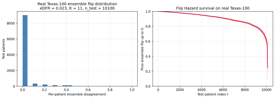
Fig. 21. Section 6.14. Real Texas-100 data. Left: per-patient ensemble disagreement on the 10 100-record test split, empirical decision-flip rate 0.0233. Right: Flip Hazard no-flip survival on the real flip stream.
