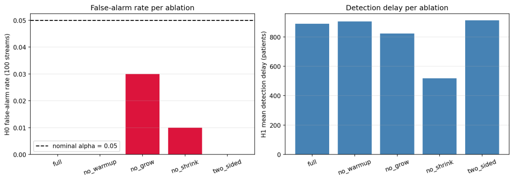
Fig. 19. Section 6.14. Module ablation. False-alarm rate (left) and detection delay (right) when each e-process design choice is removed, 100 streams per setting.
