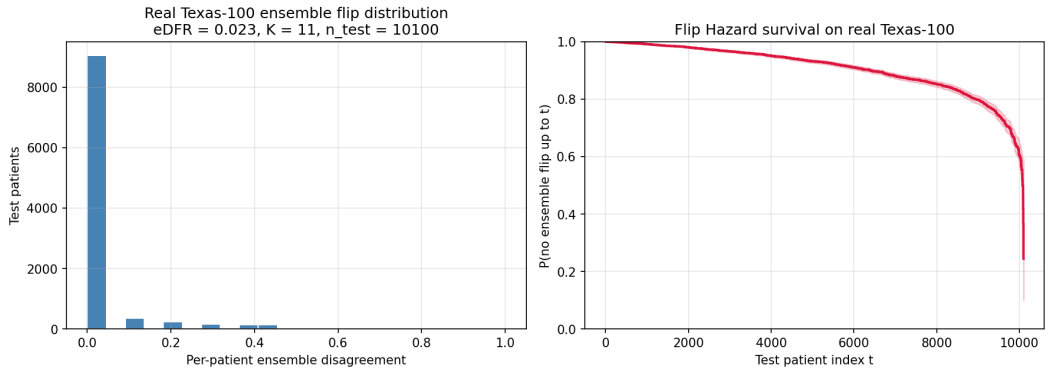
Fig. 15. Section 6.13. Real Texas-100 data. Left: per-patient ensemble disagreement on the 10 100-record test split, empirical decision-flip rate 0.0233. Right: Flip Hazard no-flip survival on the real flip stream.
