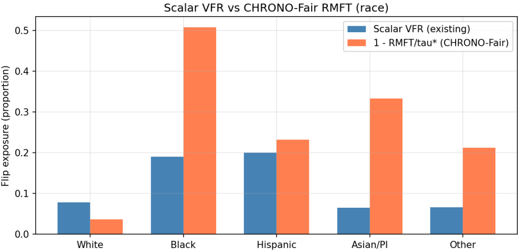
Fig. 6. Section 6.4. Scalar VFR (left bars) against 1 - \text{RMFT}/\tau^* (right bars). RMFT preserves the Black versus Hispanic ordering that the scalar VFR collapses.
