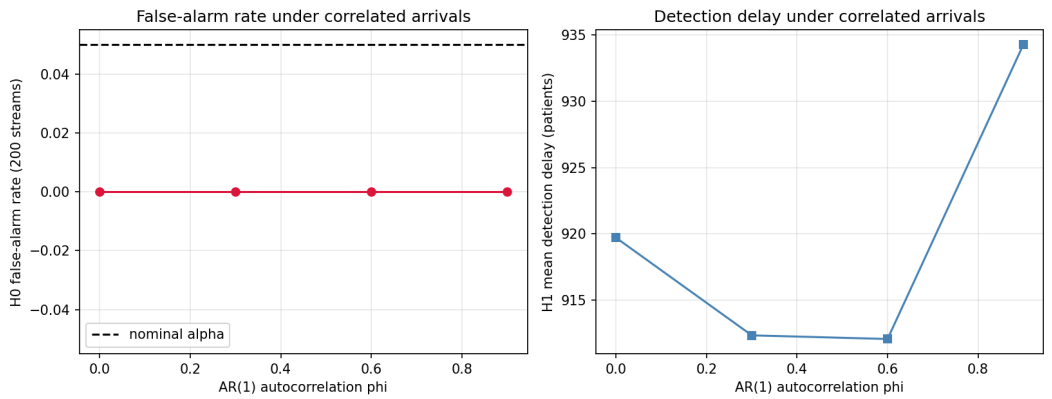
Fig. 19. Section 6.12. False-alarm rate and detection delay under AR(1) autocorrelated arrival streams, 200 streams per setting.
