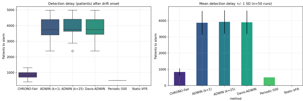
Fig. 2. Section 6.2. Detection delay across 50 Monte-Carlo runs at n = 10\,000 , drift onset at t = 5\,000 . CHRONO-Fair: 50 of 50 alarms at mean delay 837. ADWIN variants and Davis-ADWIN: 21 of 50 at mean delay 3878 to 3927. Periodic batch (500): 24 of 50 at mean 499 without peeking control. Static VFR: 0 of 50.
