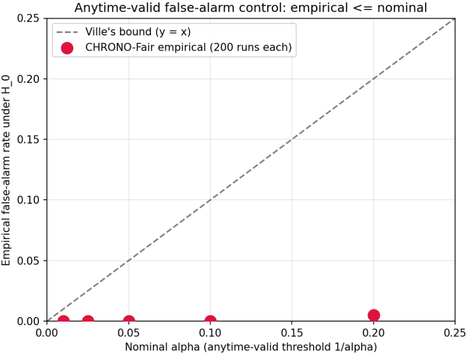
Fig. 10. Section 6.6. Empirical false-alarm rate against nominal \alpha on 200 streams per level. Points lie on or below the y = x Ville bound.
