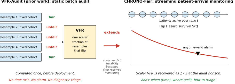
Fig. 1. VFR-Audit reports a static batch scalar. CHRONO-Fair extends the same verdict-flip object into time-resolved monitoring with an alarm and diagnostic triage.
