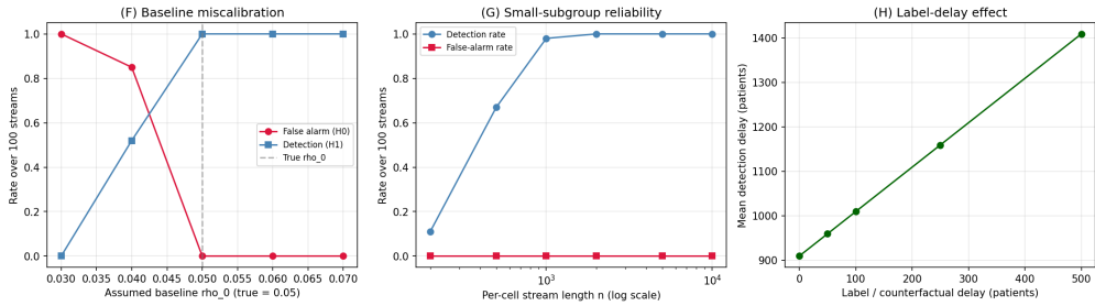
Fig. 16. Section 6.13. Robustness stress tests, 100 streams per setting. Left: baseline miscalibration; underestimating \rho_0 inflates false alarms, overestimating only delays detection. Centre: small-subgroup reliability; the detection rate exceeds 0.95 once the per-cell stream reaches roughly 1000 patients. Right: label delay adds linearly to the wall-clock detection delay.
