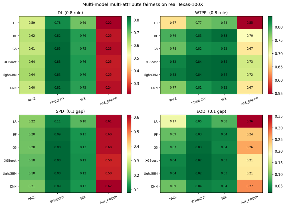
Fig. 13. Section 6.9. Multi-model multi-attribute fairness on real Texas-100X. Each panel is one metric (DI, WTPR, SPD, EOD) across six models and four protected attributes. Cell value is the metric; colour encodes pass-or-fail under the 0.8 rule for the ratio metrics and the 0.1 gap rule for SPD/EOD.
