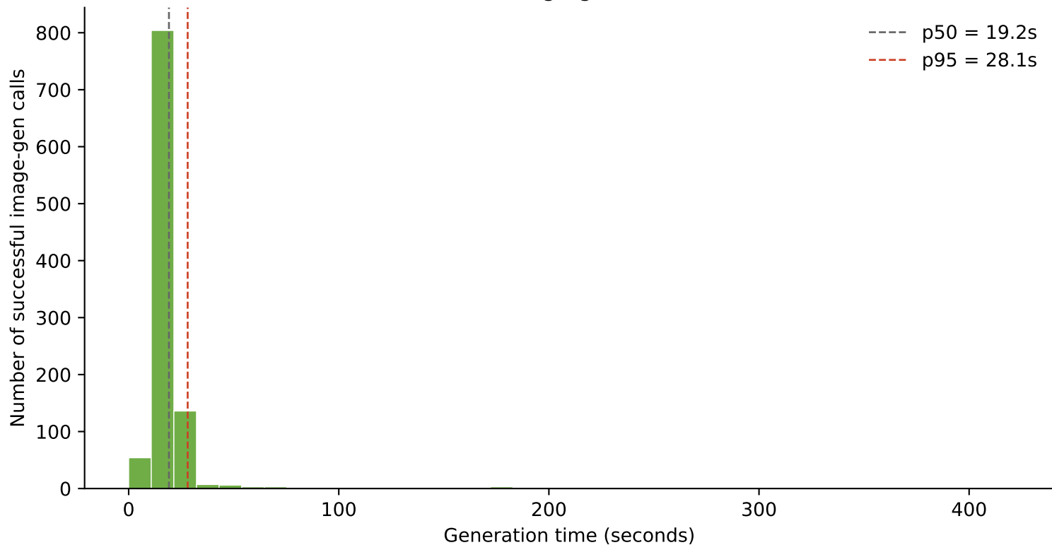
Distribution of successful image-generation durations (n=1038)
