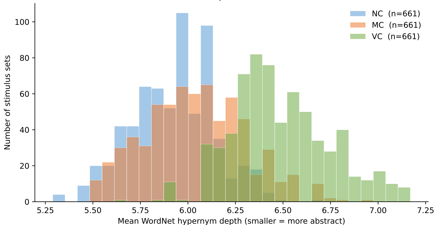
Distribution of WordNet mean per condition (n=661 stimulus sets)
