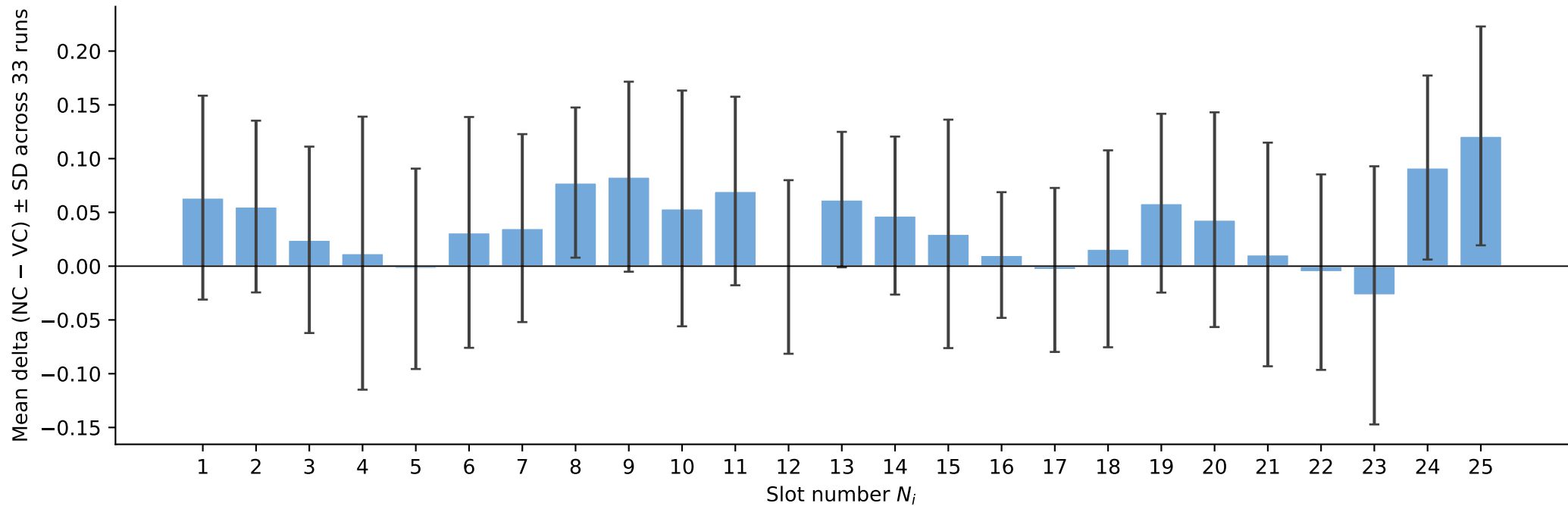
RQ2 — per-slot mean abstraction delta across all 33 source runs
