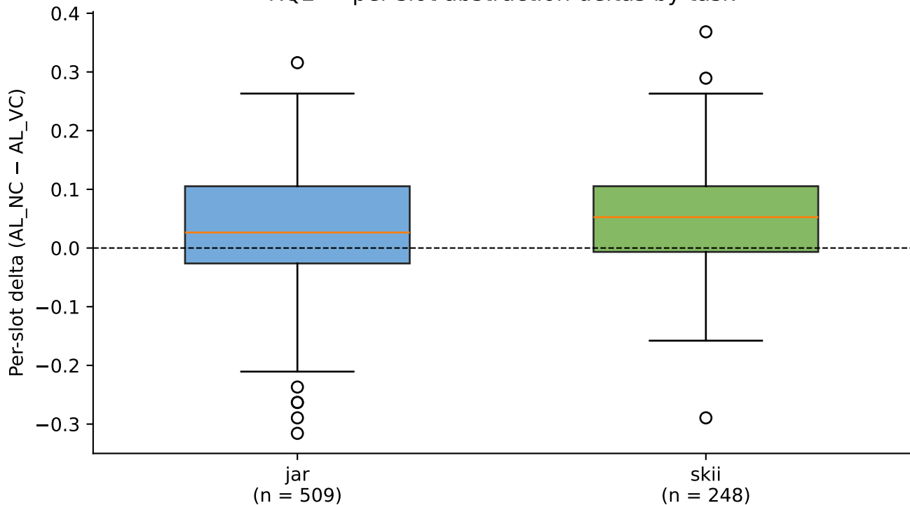
RQ2 — per-slot abstraction deltas by task
