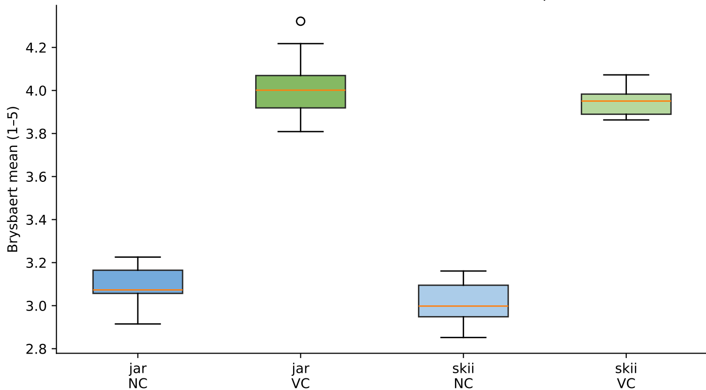
Per-task NC vs VC concreteness — final corpus
