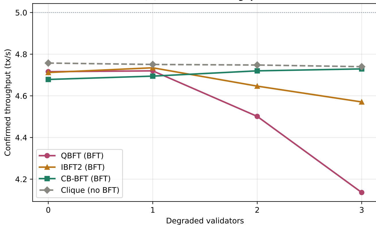
(b) Confirmed throughput
