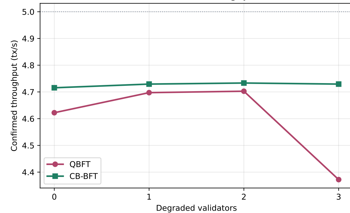
(c) Confirmed throughput
