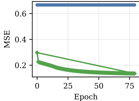
ECG — Loss
