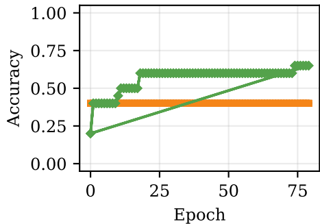
ECG — Accuracy
