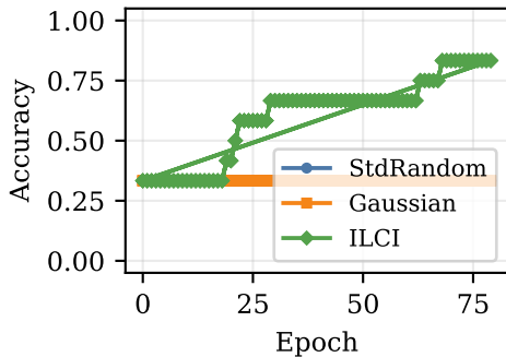
Iris — Accuracy
