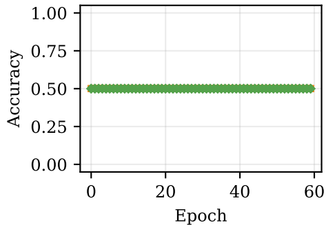
XOR — Accuracy
