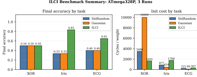
Fig. 3. Benchmark summary: final accuracy and cycles per weight by task.
