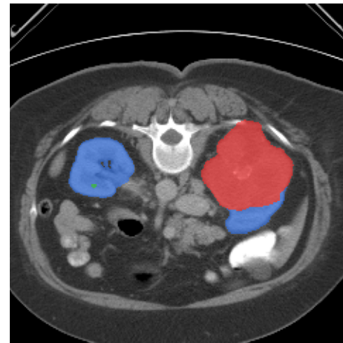
WaLM-Net
