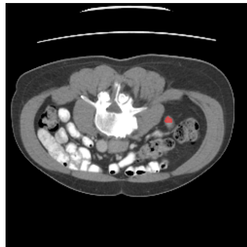
WaLM-Net
