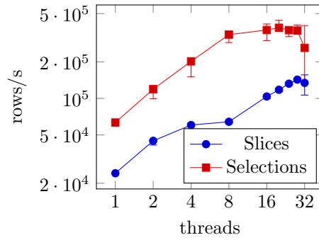
Figure 1: Parallel scaling of the memory-bound benchmarks.
