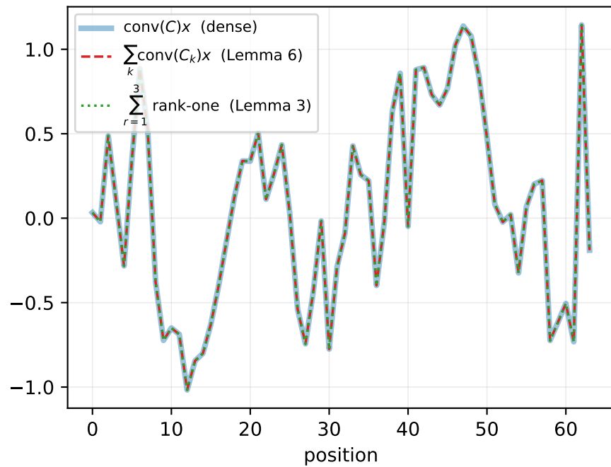
(b) reconstruction, max error 5.6\text{e-}16
