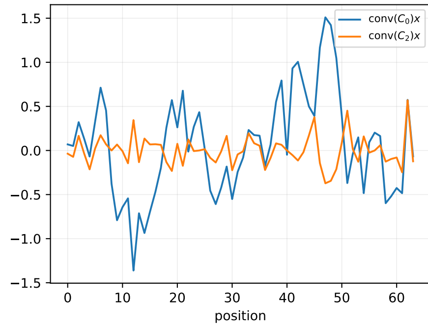
(a) Lemma 6: only k \in \{0, 2\} contribute
