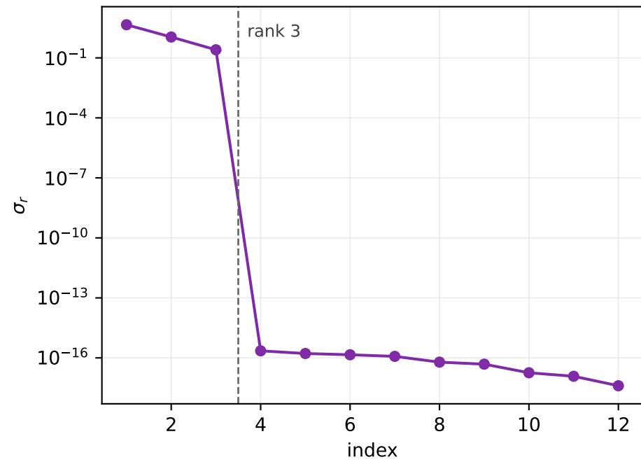
(c) singular values of C : exactly three nonzero
