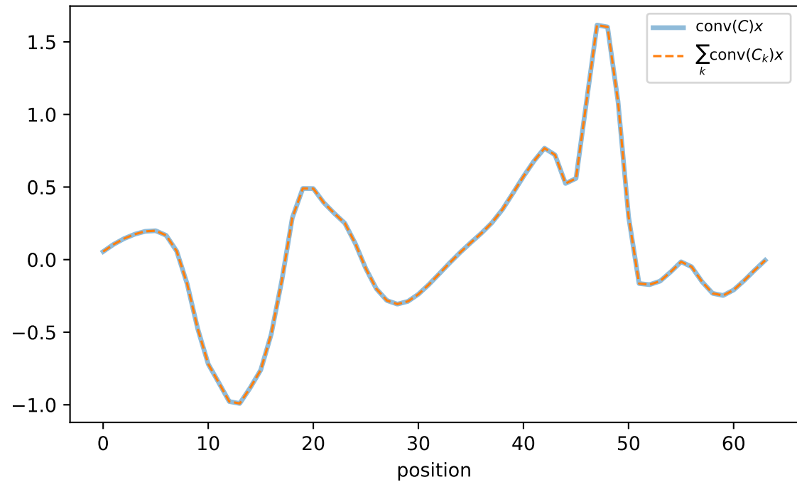
reconstruction, max error 6.66e-16
