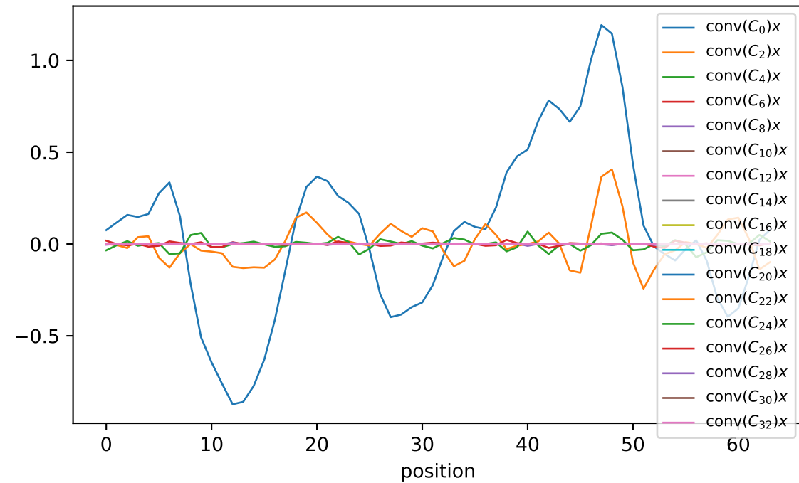
frequency-selective contributions (Lemma 6)
