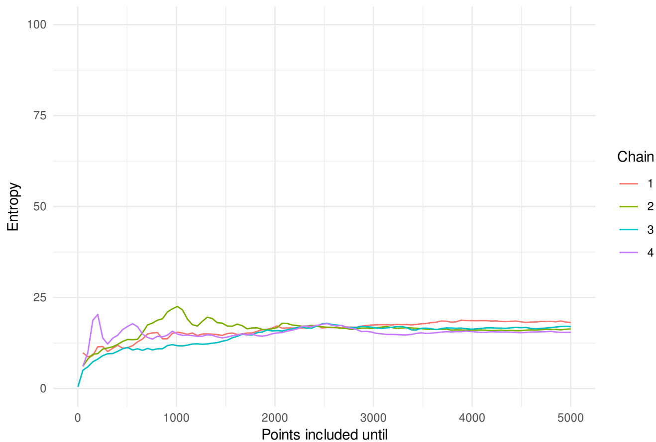
Entropy along the Chain in 3 dimensions
