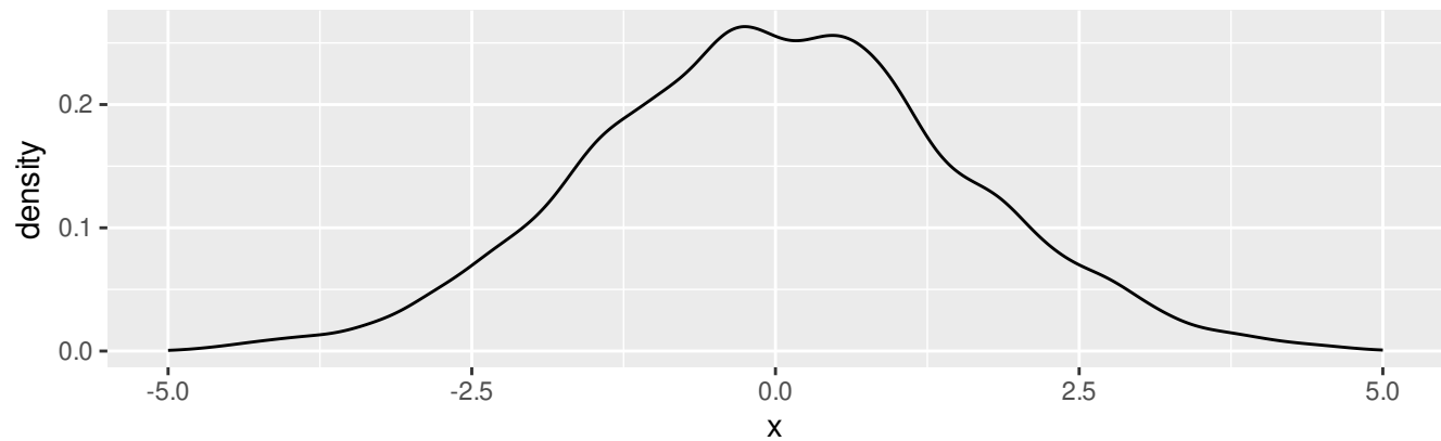
Posterior of MCMC with 10000 samples
