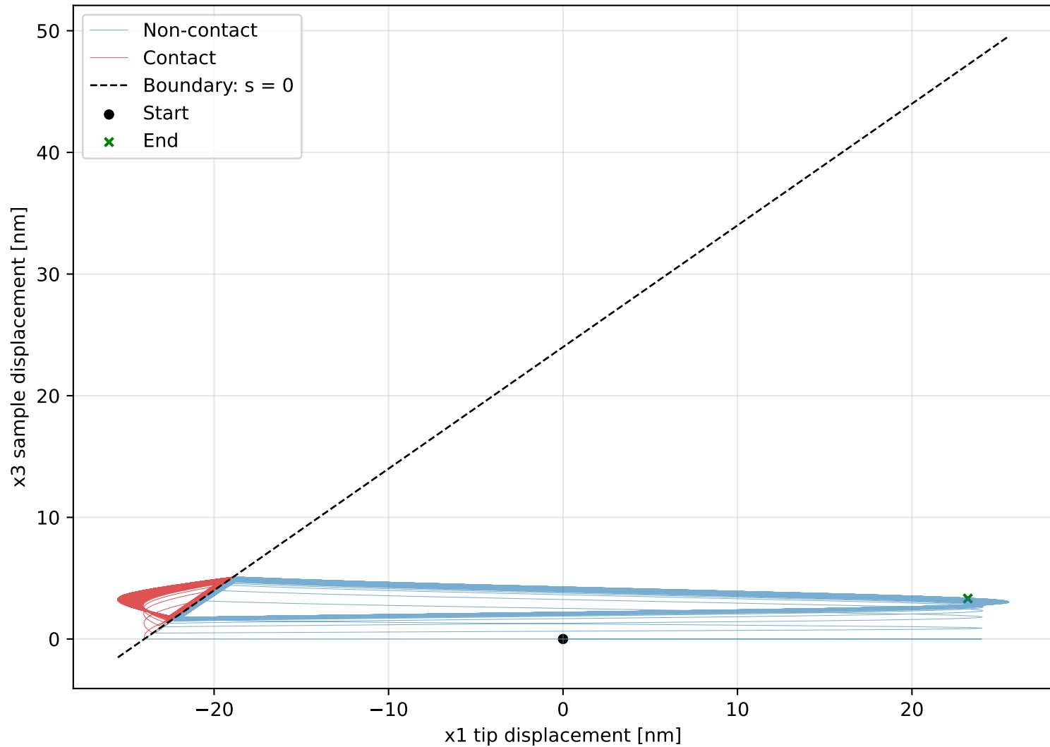
AFM DMT-KV Phase Space: x_1 vs x_3 (Full Trajectory)
