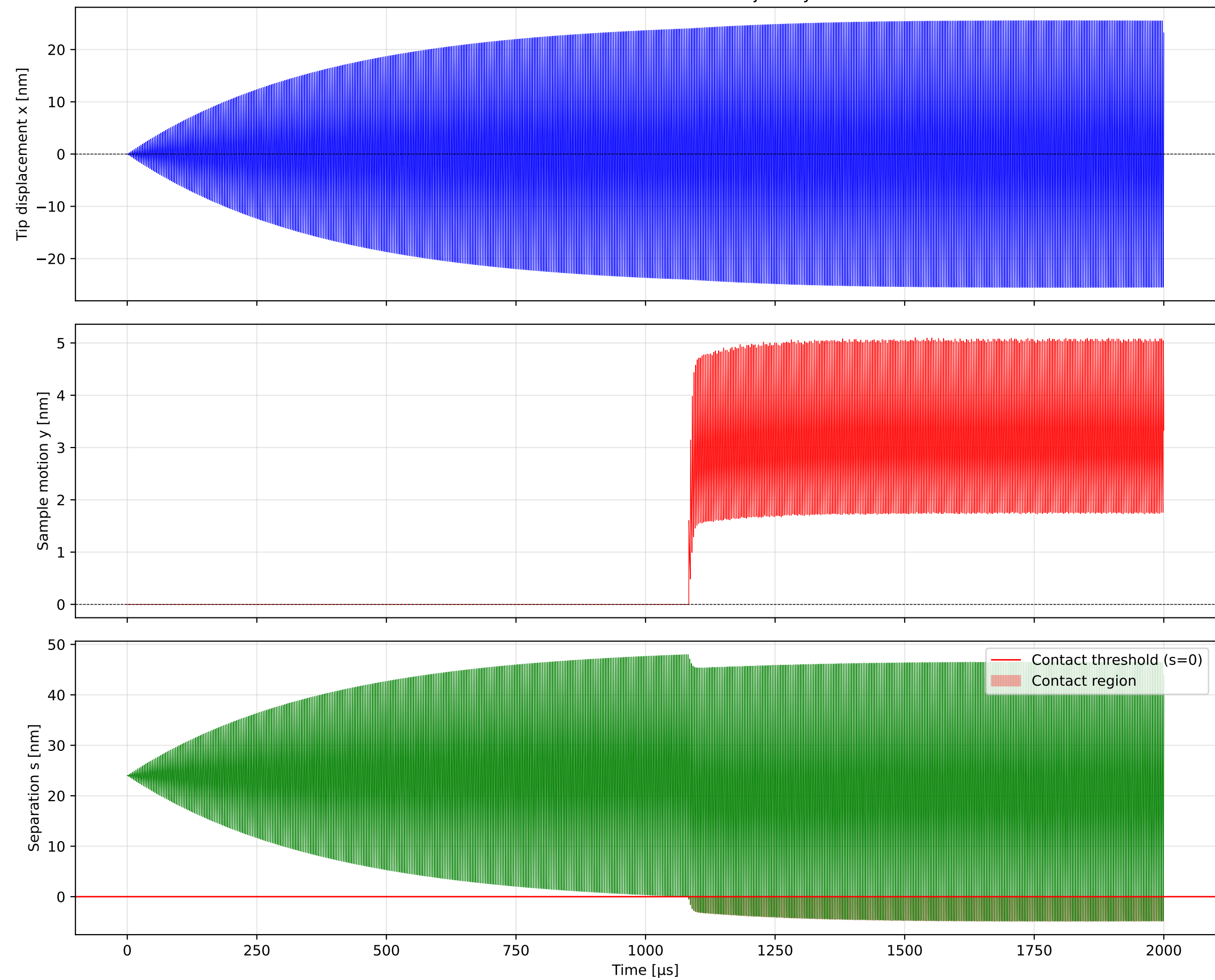
AFM DMT-KV Simulation: Full Trajectory
