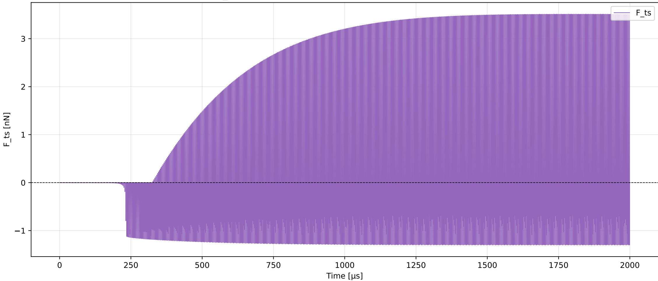
AFM DMT-KV F_ts Time-Domain Signal (sigmoid-gated unified DMT-like force in s)
