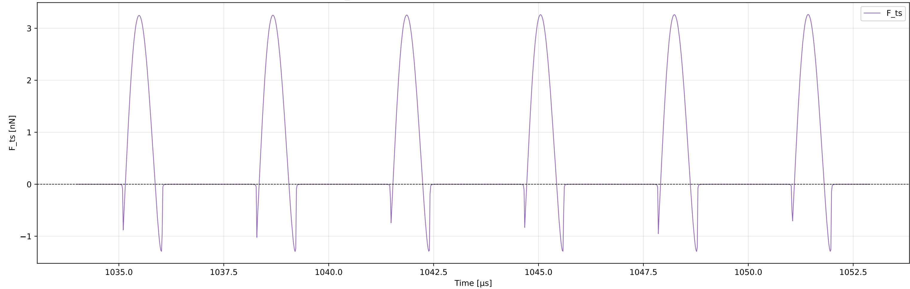
AFM DMT-KV F ts Time-Domain Signal (long window from W1 start, 1182 samples)
