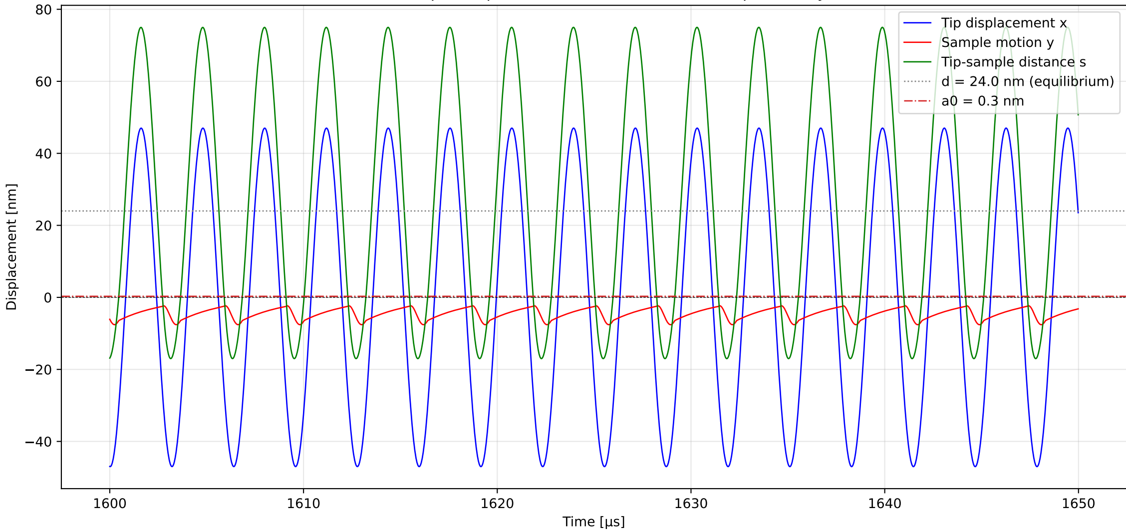
AFM DMT-KV: Tip, Sample, and Distance s (1600-1650 \mu\text{s} , Steady-State)
