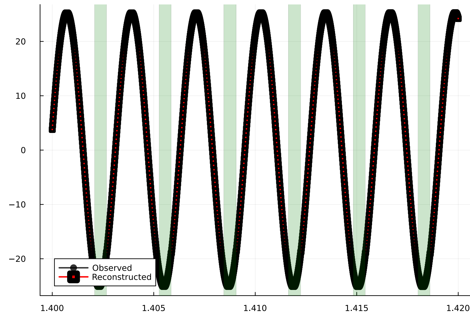
Tip Displacement - Detail (1.4000-1.4200 ms)
