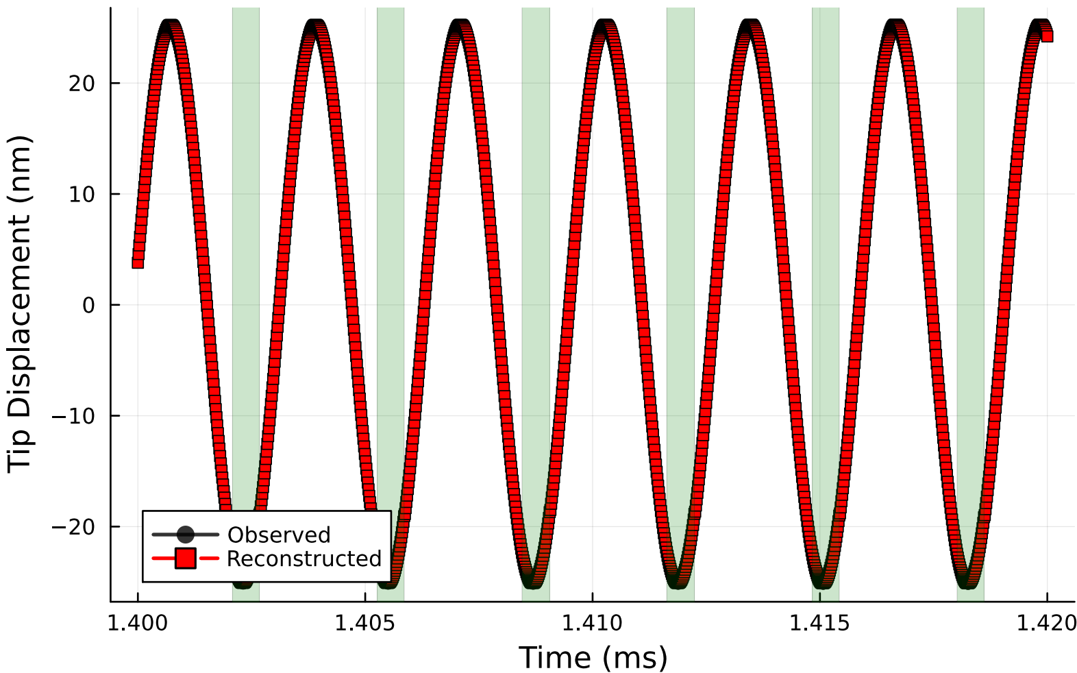
Tip Displacement - Detail (1.4000-1.4200 ms)
